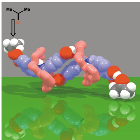
Fig. 10 Despite the formation of a carboxylic acid dimer between individual [2]pseudorotaxanes, the possibility of an infinite hydrogen bonded polymer is negated by the formation of hydrogen bonds from the terminal carboxylic acid protons to included acetone molecules in the solid-state superstructure of [DB24C8·5] + .
