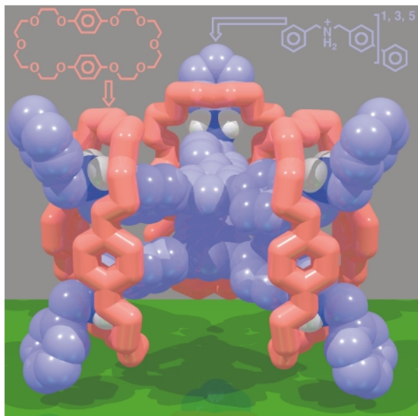
Fig. 29 The solid-state superstructure of the five-component superbundle [(\text{BPP34C10})_3 \cdot (\mathbf{8})_2]^{6+} formed between the trifurcated tris(ammonium) cation \mathbf{8}^{3+} and the ditopic crown ether BPP34C10.
