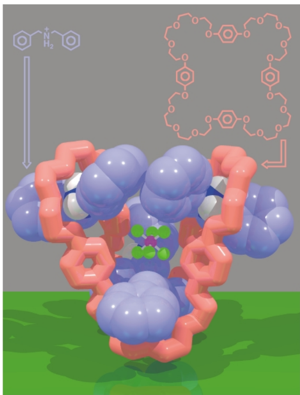
Fig. 39 The extended crown ether TPP68C20 co-crystallises with four equivalents of DBA·PF 6 to give a quadruple-threaded [5]pseudorotaxane [TPP68C20·(DBA) 4 ] 4+ . One PF 6 − anion is encapsulated completely within the superstructure.
