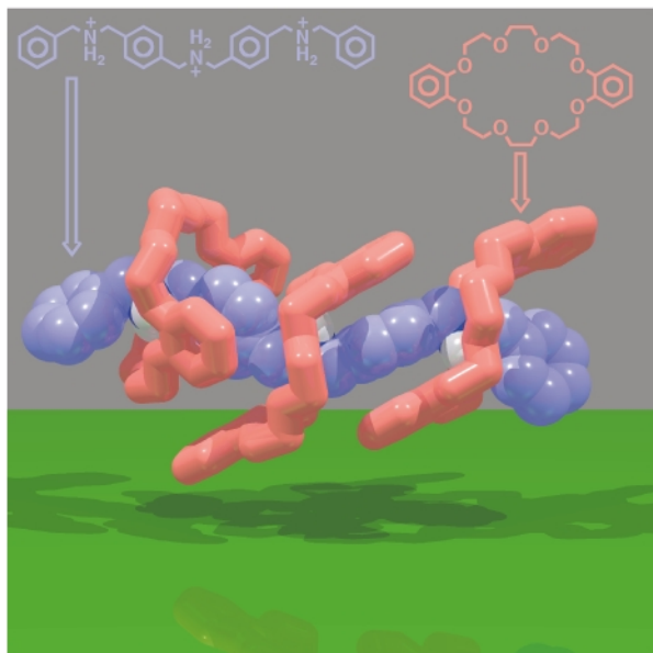
Fig. 5 The solid-state superstructure of a [4]pseudorotaxane [(DB24C8) 3 ·2] 3+ formed between a thread-like molecule—containing three ammonium centres (2·3PF 6 )—and three DB24C8 macrocycles.
