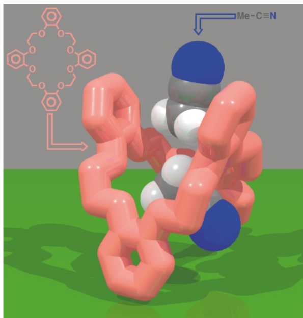
Fig. 15 When grown from a MeCN/Et 2 O solution, crystals of TB24C8 can be seen to contain enclathrated acetonitrile molecules.
