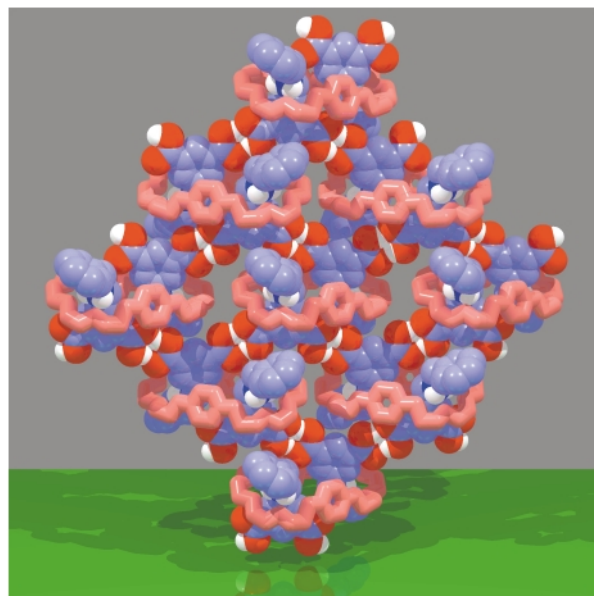
Fig. 37 Analysis of the extended solid-state superstructure adopted by [\text{BPP34C10} \cdot (7)_2]^{3+} reveals the existence of an interwoven cross-linked supramolecular polymer.
