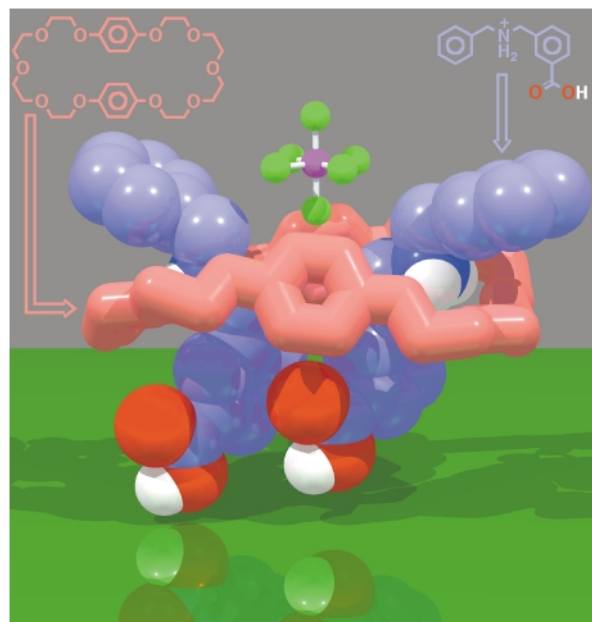
Fig. 34 Similarly to 4 \cdot \text{PF}_6 , its meta -substituted cousin 10 \cdot \text{PF}_6 forms a 1:2 complex when co-crystallised with BPP34C10.
