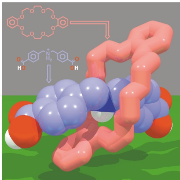
Fig. 9 The solid-state superstructure of the [2]pseudorotaxane [DB24C8·5] + formed between the bis( para -carboxylic acid)-substituted DBA + cation 5 + and DB24C8.
