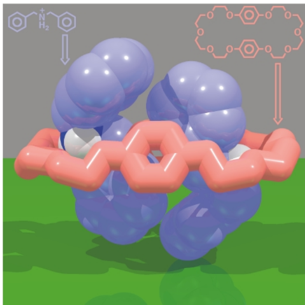
Fig. 25 The solid-state superstructure of a double-stranded [3]pseudorotaxane [\text{BPP34C10} \cdot (\text{DBA})_2]^{2+} formed between BPP34C10 and \text{DBA} \cdot \text{PF}_6^- .
