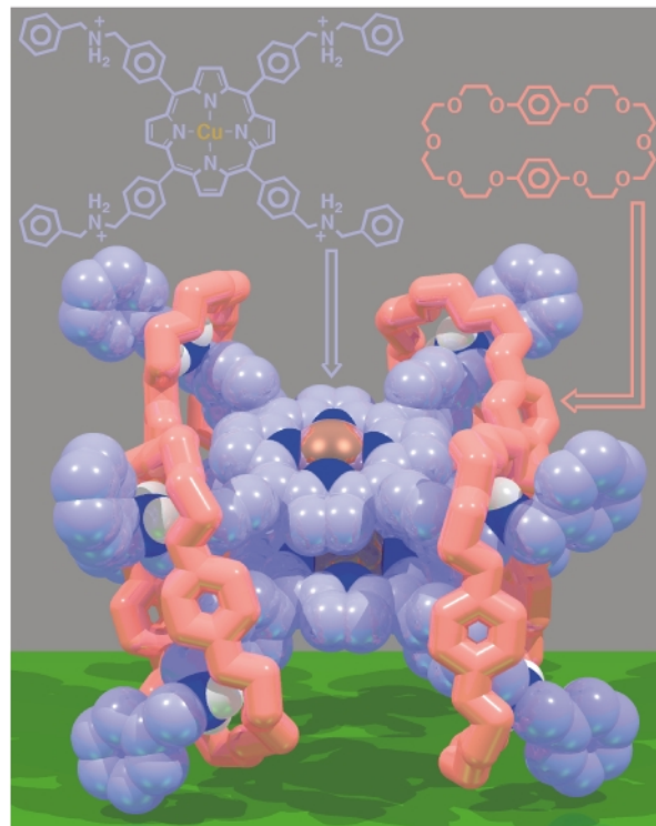
Fig. 31 Co-crystallisation of BPP34C10 and \mathbf{9} \cdot 4\text{PF}_6 affords a six-component superbundle that is a supramolecular analogue of the photosynthetic special pair.
