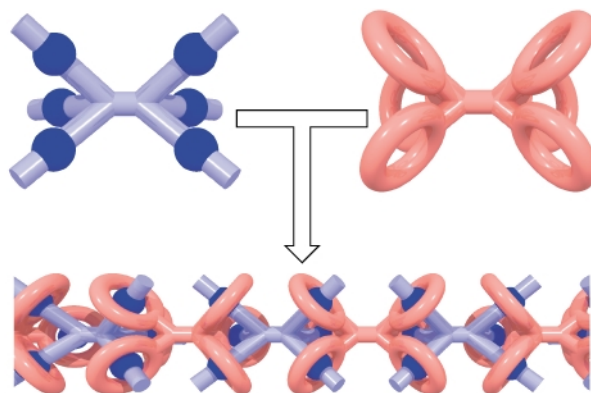
Fig. 44 A schematic representation of supramolecular polymer formation anticipated upon mixing a monomer containing two tris(DB24C8) units with another that contains two trifurcated tris(ammonium) cation clusters.
