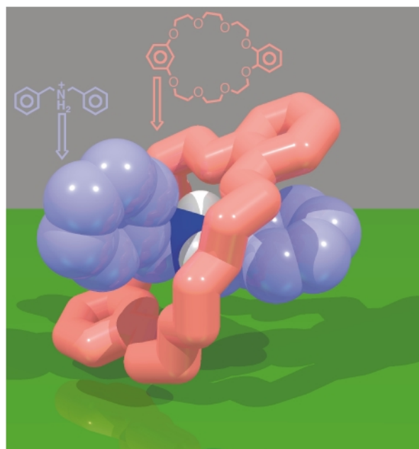
Fig. 19 The solid-state superstructure of the [2]pseudorotaxane [BMP25C8·DBA] + formed between the DBA + cation and BMP25C8.
