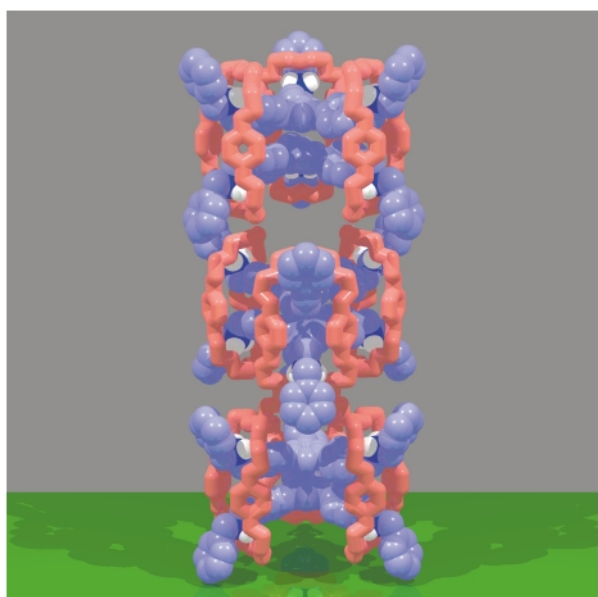
Fig. 30 Interleaved one-dimensional arrays of the five-component superbundle [(\text{BPP34C10})_3 \cdot (\mathbf{8})_2]^{6+} are formed in the solid state.
