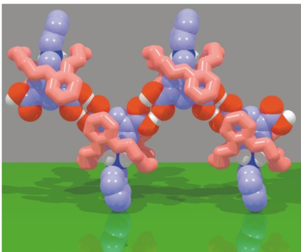
Fig. 14 The side-chain pseudopolyrotaxane formed as a result of carboxylic acid dimerisation in the extended superstructure of [DB24C8·7] + .
