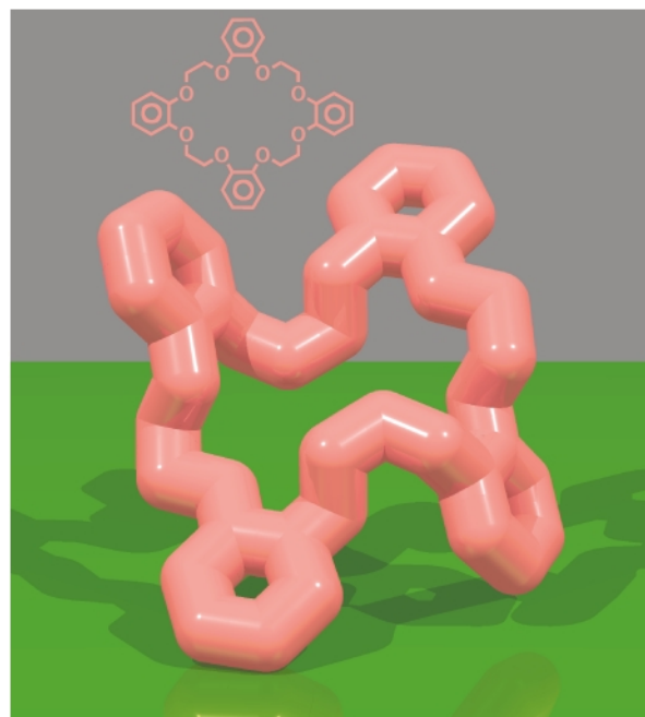
Fig. 16 In the absence of MeCN, the crown ether TB24C8 crystallises without ordered solvent molecules.
