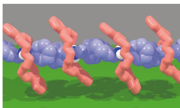
Fig. 3 \pi - \pi Stacking of the benzyl rings of the [2]pseudorotaxane [(\text{DB24C8} \cdot \text{DBA})]^+ produces an infinite linear pseudopolyrotaxane.
