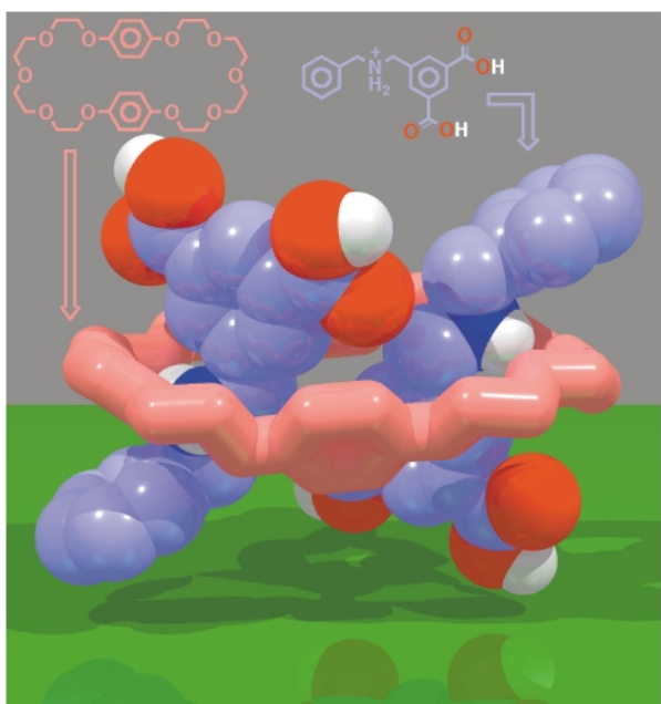
Fig. 36 Two 7^+ cations thread through the cavity of BPP34C10 in a centrosymmetric fashion, resulting in the formation of a [3] pseudorotaxane [\text{BPP34C10} \cdot (7)_2]^{2+} in the solid state.
