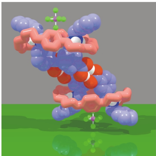
Fig. 35 Discrete [\text{BPP34C10} \cdot (10)_2][2\text{PF}_6] supermolecules dimerise—in the solid-state—as a result of carboxyl dimer formation.
