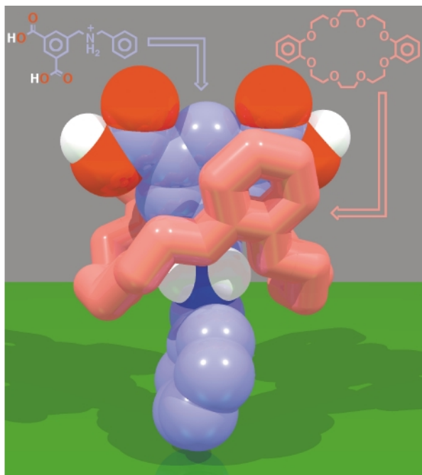
Fig. 13 The solid-state superstructure of the [2]pseudorotaxane [DB24C8·7] + formed between the isophthalic acid-substituted DBA + cation 7 + and DB24C8.
