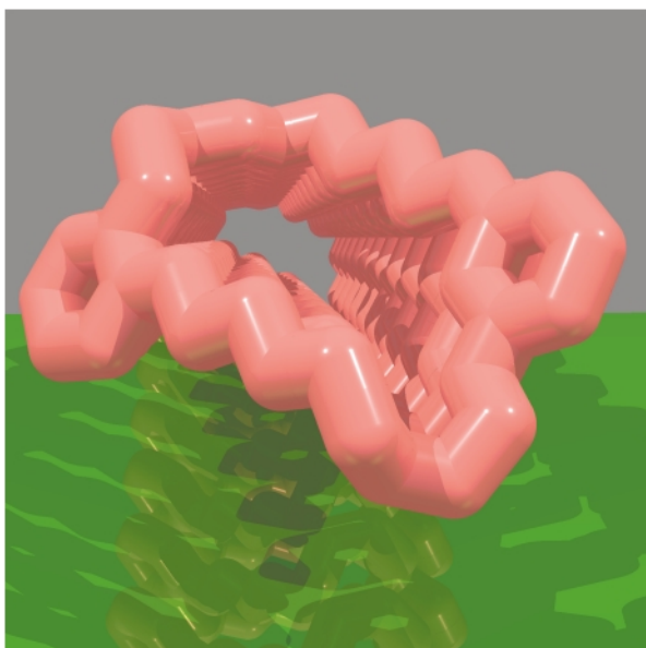
Fig. 22 Constricted nanotubes—stabilised by intermolecular C–H...O hydrogen bonds—are formed by the stacking of BMP25C8 molecules in the solid state.
