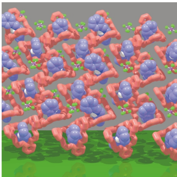
Fig. 18 The extensively C–H···F hydrogen bond-stabilised extended superstructure of the complex [TB24C8·DBA][PF 6 ].
