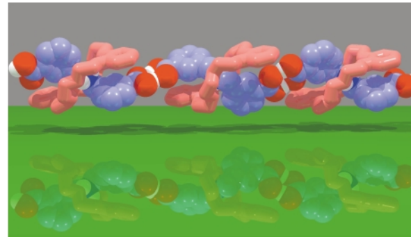
Fig. 12 The X-ray crystallographic analysis of [DB24C8·6][PF 6 ] reveals the formation—in the solid state—of a carboxyl-dimer-linked main chain pseudopolyrotaxane.
