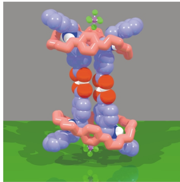
Fig. 33 Individual [\text{BPP34C10} \cdot (4)_2][2\text{PF}_6] [3]pseudorotaxanes dimerise in the solid state via the formation of carboxylic acid dimers.
