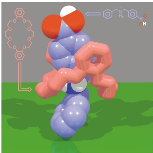
Fig. 7 The solid-state superstructure of the [2]pseudorotaxane [DB24C8·4] + formed between the para -carboxylic acid-substituted DBA + cation 4 + and DB24C8.
