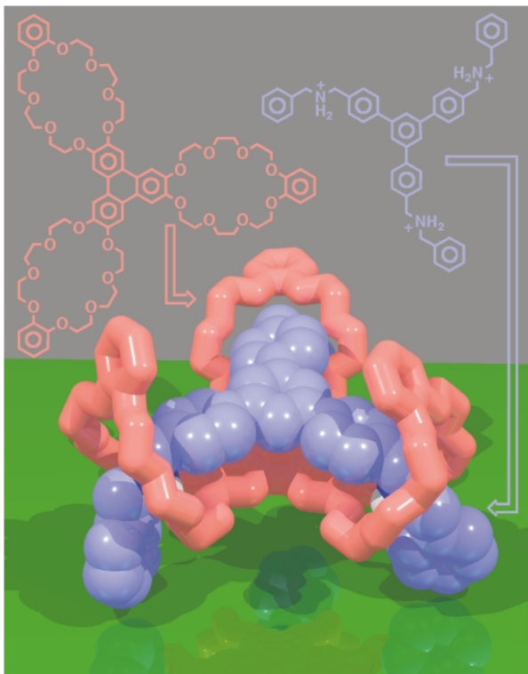
Fig. 43 The solid-state superstructure of a triple-threaded 1:1 complex formed between a trifurcated tris(ammonium) thread and a complementary triphenylene-based tris(DB24C8) derivative.
