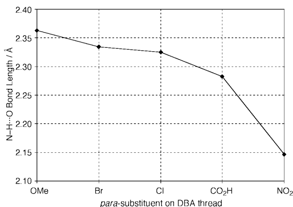
Fig. 46 A graph showing how \text{N}^+-\text{H}\cdots\text{O} hydrogen bond distance decreases as the \text{DBA}^+ benzyl group is functionalised with increasingly electron-withdrawing substituents.
