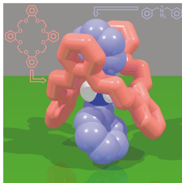
Fig. 17 One of the four crystallographically independent superstructures with a [2]pseudorotaxane geometry observed in the X-ray analysis of [TB24C8·DBA][PF 6 ].
