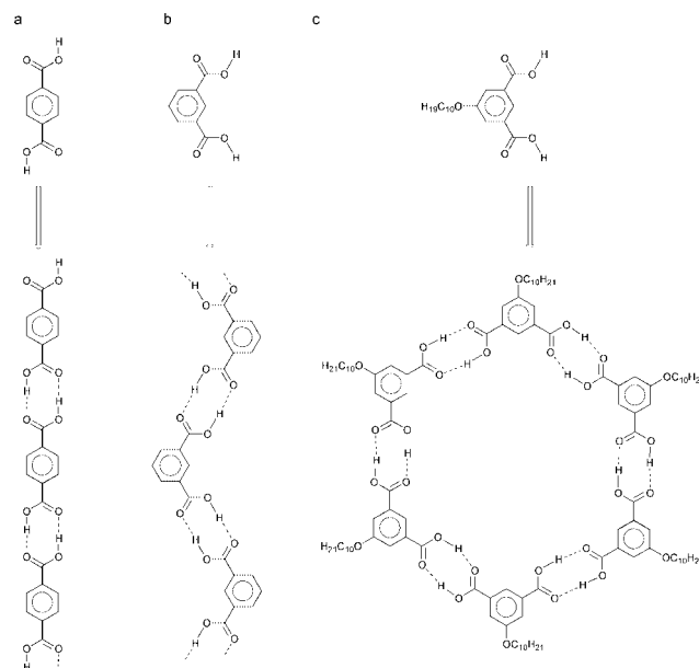
Fig. 6 The influence of both directionality and steric crowding upon solid-state superstructures assembled via the carboxylic acid dimer are highlighted. The para disposition of carboxylic acid groups in terephthalic acid (a) results in the formation of infinite linear tapes, whereas the meta disposition—as in isophthalic acid (b)—produces a crinkled tape. The sterically congested 5-decyloxyisophthalic acid (c) is precluded from forming an extended tape superstructure, assembling instead into discrete hexameric supramacrocycles.
