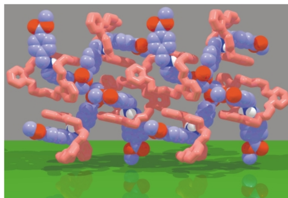
Fig. 24 The extended superstructure of [TB27C9·( p -CO 2 Me) 2 -DBA][PF 6 ] consists of extended sheets that are stabilised by inter-[2]pseudorotaxane C–H...π hydrogen bonds.
