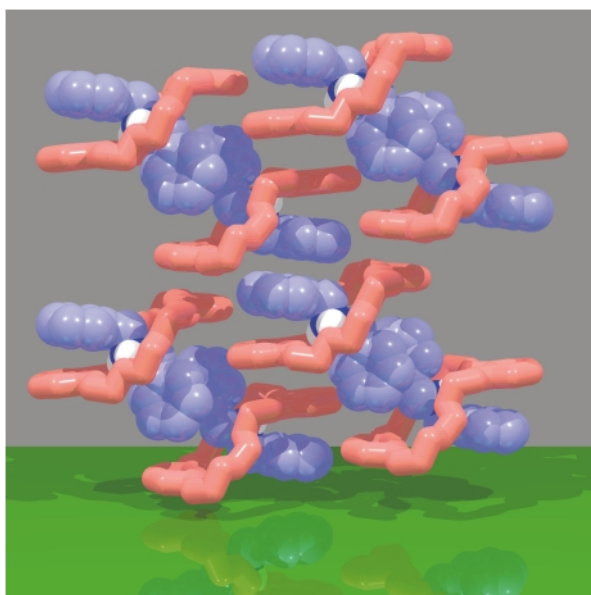
Fig. 20 Discrete [BMP25C8·DBA] + supermolecules are linked in the solid state to form extended sheets.
