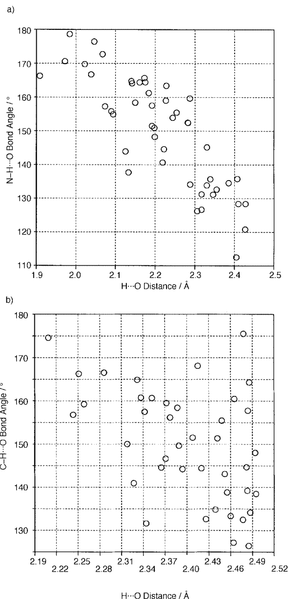
Fig. 45 a) Scatterplot of \text{N}^+-\text{H}\cdots\text{O} bond angles and \text{H}\cdots\text{O} bond distances observed in the solid state for all DB24C8-derived ammonium-based rotaxanes and pseudorotaxanes; b) a similar scatterplot relating the \text{C}-\text{H}\cdots\text{O} bond angles and \text{H}\cdots\text{O} bond distances observed in the solid state.
