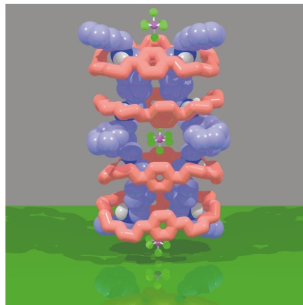
Fig. 28 Individual [2 + 2] superbundles form columns in the solid state. The interstitial \text{PF}_6^- anions may play some role in the assembly of this infinite one-dimensional array.
