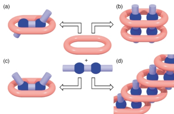
Fig. 26 Conceivably, there are four possible distinct superstructures that may form upon co-crystallisation of BPP34C10 and 1 \cdot 2\text{PF}_6^- : (a) a single-threaded, double-docked [2]pseudorotaxane, (b) a double-threaded, double-encircled [4]pseudorotaxane, (c) a face-to-face complex, and (d) a polymer .
