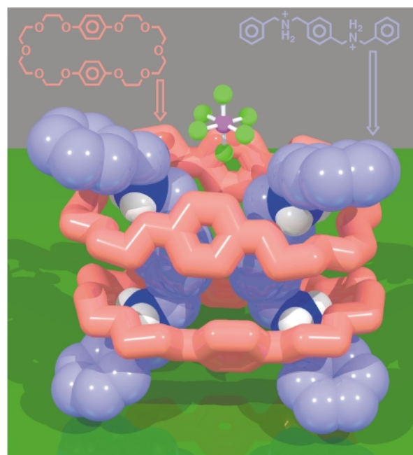
Fig. 27 The solid-state superstructure of the double-threaded, double-encircled [4]pseudorotaxane [(\text{BPP34C10})_2 \cdot (1)_2]^{4+} formed between BPP34C10 and 1^{2+} .
