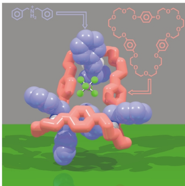
Fig. 38 The extended crown ether TPP51C15 co-crystallises with three equivalents of \text{DBA} \cdot \text{PF}_6 to give a triple-threaded [4] pseudorotaxane [\text{TPP51C15} \cdot (\text{DBA})_3]^{3+} . Note how a \text{PF}_6^- anion occupies a cleft in the superstructure.
