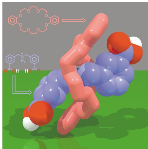
Fig. 11 The solid-state superstructure of the [2]pseudorotaxane [DB24C8·6] + formed between the bis( meta -carboxylic acid)-substituted DBA + cation 6 + and DB24C8.
