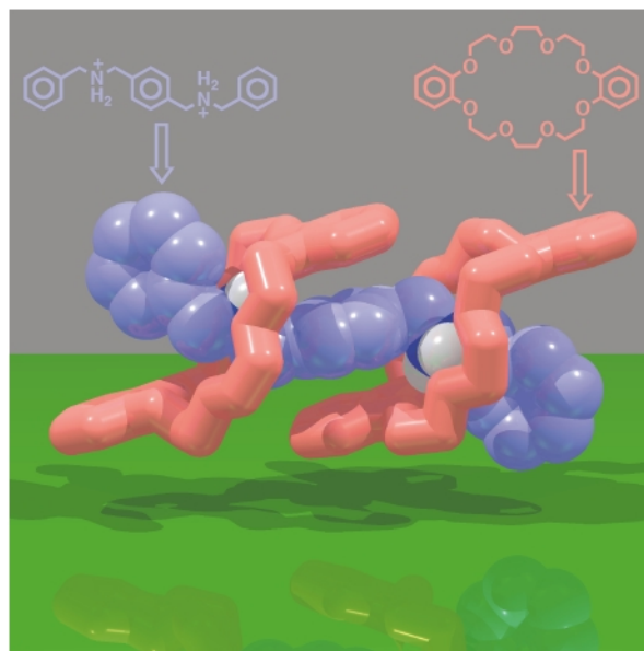
Fig. 4 The solid-state superstructure of a [3]pseudorotaxane [(\text{DB24C8})_2 \cdot 1]^{2+} formed between a thread-like molecule—containing two ammonium centres ( 1 \cdot 2\text{PF}_6 )—and two DB24C8 macrocycles.
