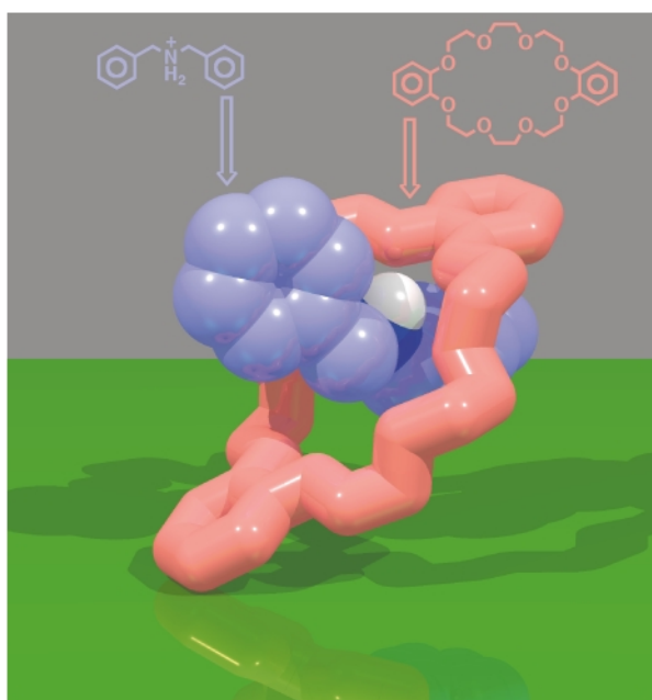
Fig. 2 One of the two distinct superstructures adopted in the solid state by the [2]pseudorotaxane [(\text{DB24C8} \cdot \text{DBA})]^+ .
