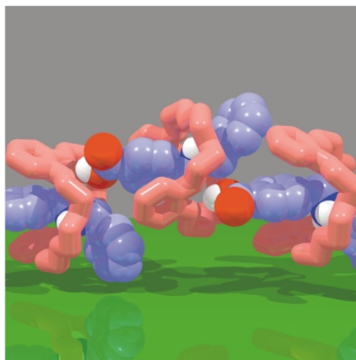
Fig. 8 An infinite linear daisy-chain-like array of [DB24C8·4] + is formed as a result of hydrogen bonding between the carboxylic acid of one thread and the crown ether component of a neighbouring [2]pseudorotaxane.
