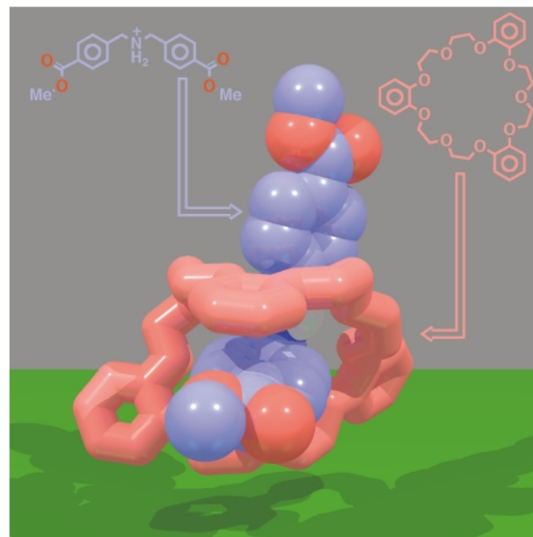
Fig. 23 The solid-state superstructure of the [2]pseudorotaxane [TB27C9·( p -CO 2 Me) 2 -DBA] + formed between the p -CO 2 Me-disubstituted DBA + cation and TB27C9.
